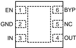
MIC5255-x.xBML 6-Pin 2mm × 2mm MLF™ (ML) (Top View)
