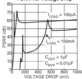
PSRR vs. Voltage Drop
