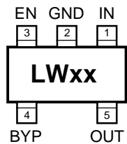
MIC5255-x.xBM5 (SOT-23-5)
