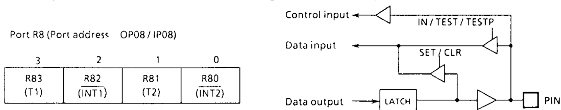
Figure 3-5. Port R8
