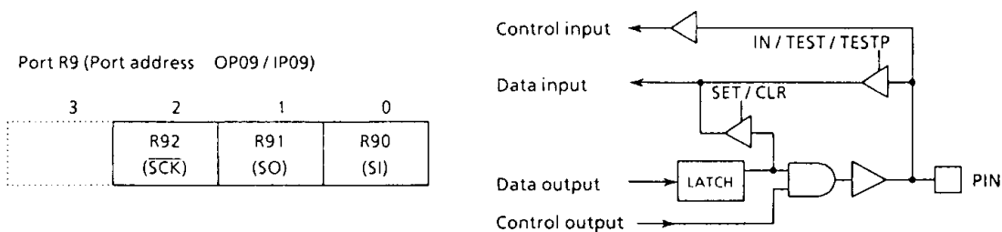
Figure 3-6. Port R9
