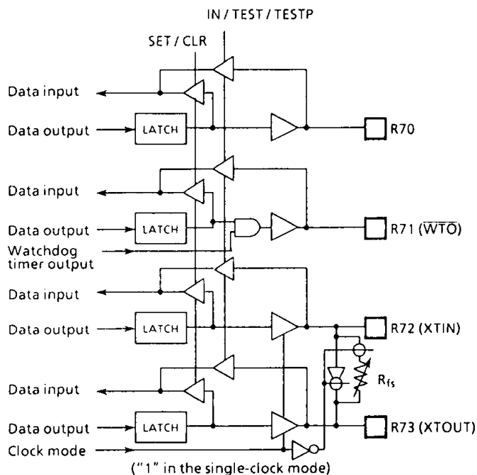
Figure 3-4. Port R7
