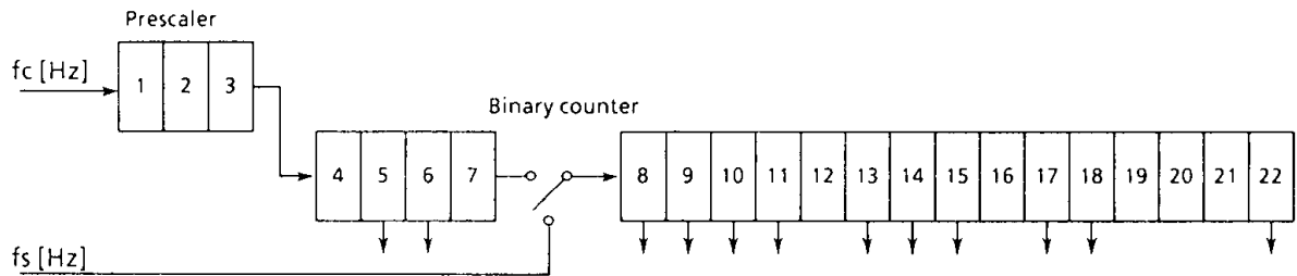
Figure 3-10. Configuration of Interval Timer
