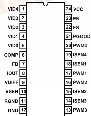
ISL6557 24 PIN (SOIC) TOP VIEW
