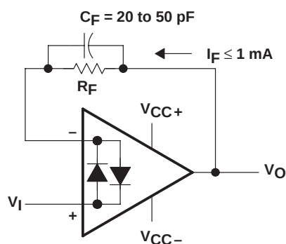
Figure 53. Voltage-Follower Circuit
