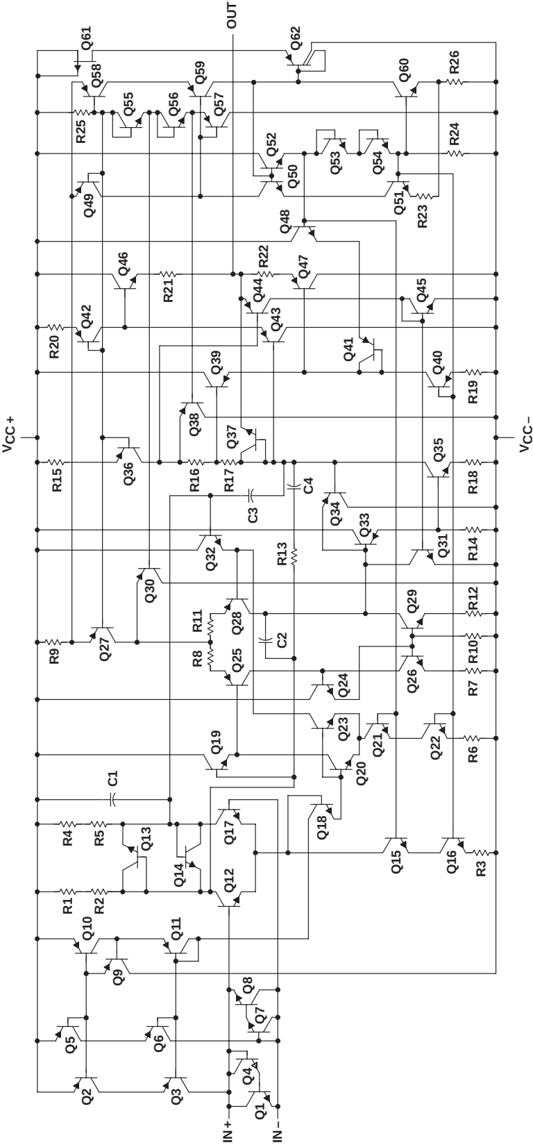
equivalent schematic (each amplifier)
