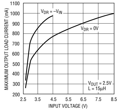
Maximum Output Load Current vs Input Voltage
