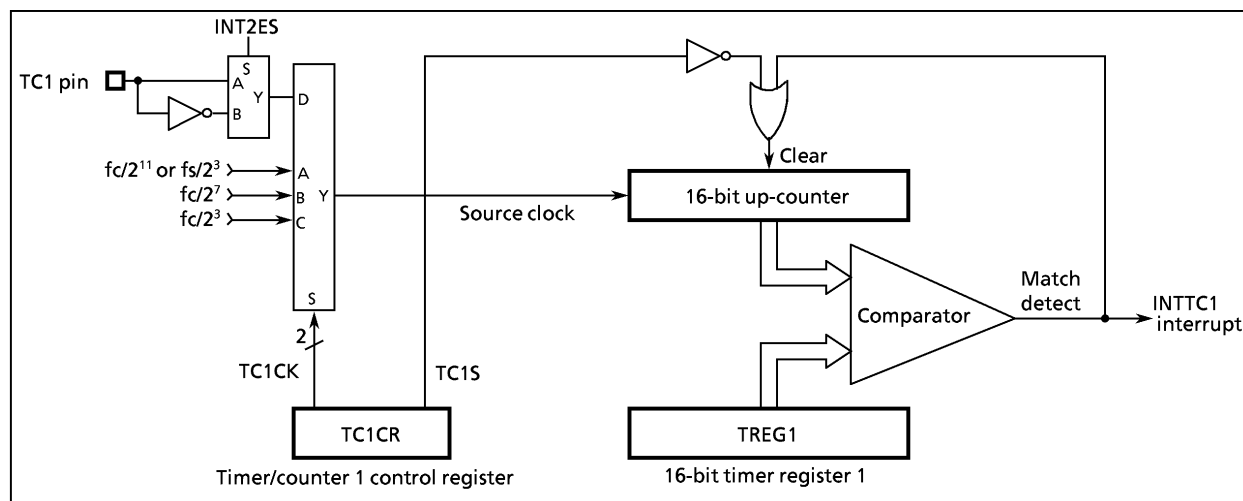
Figure 2-16. Timer/Couter 1
