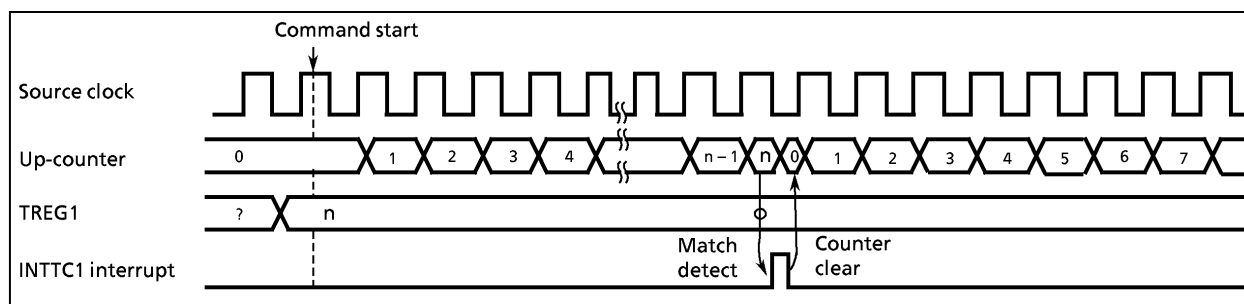
Figure 2-18. Timer Mode Timing Chart
