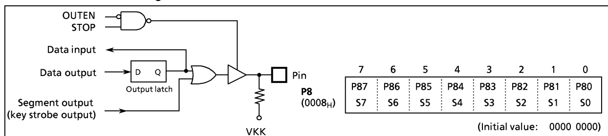
Figure 2-10. Port P8
