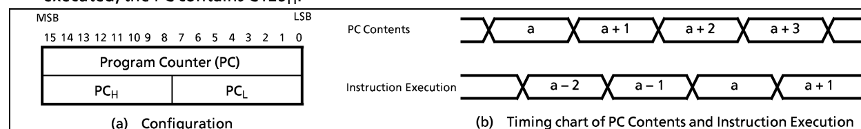
Figure 1-3. Program Counter
