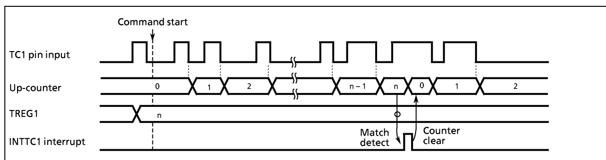
Figure 2-19. Event Counter Mode Timing Chart (INT2ES = 1)
