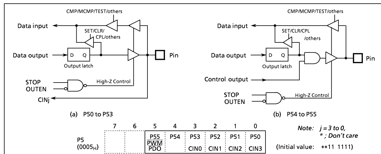
Figure 2-8. P5 Port
