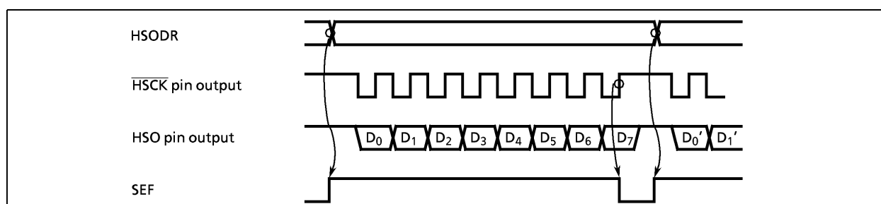
Figure 2-40. High-speed Serial Output Timing Chart
