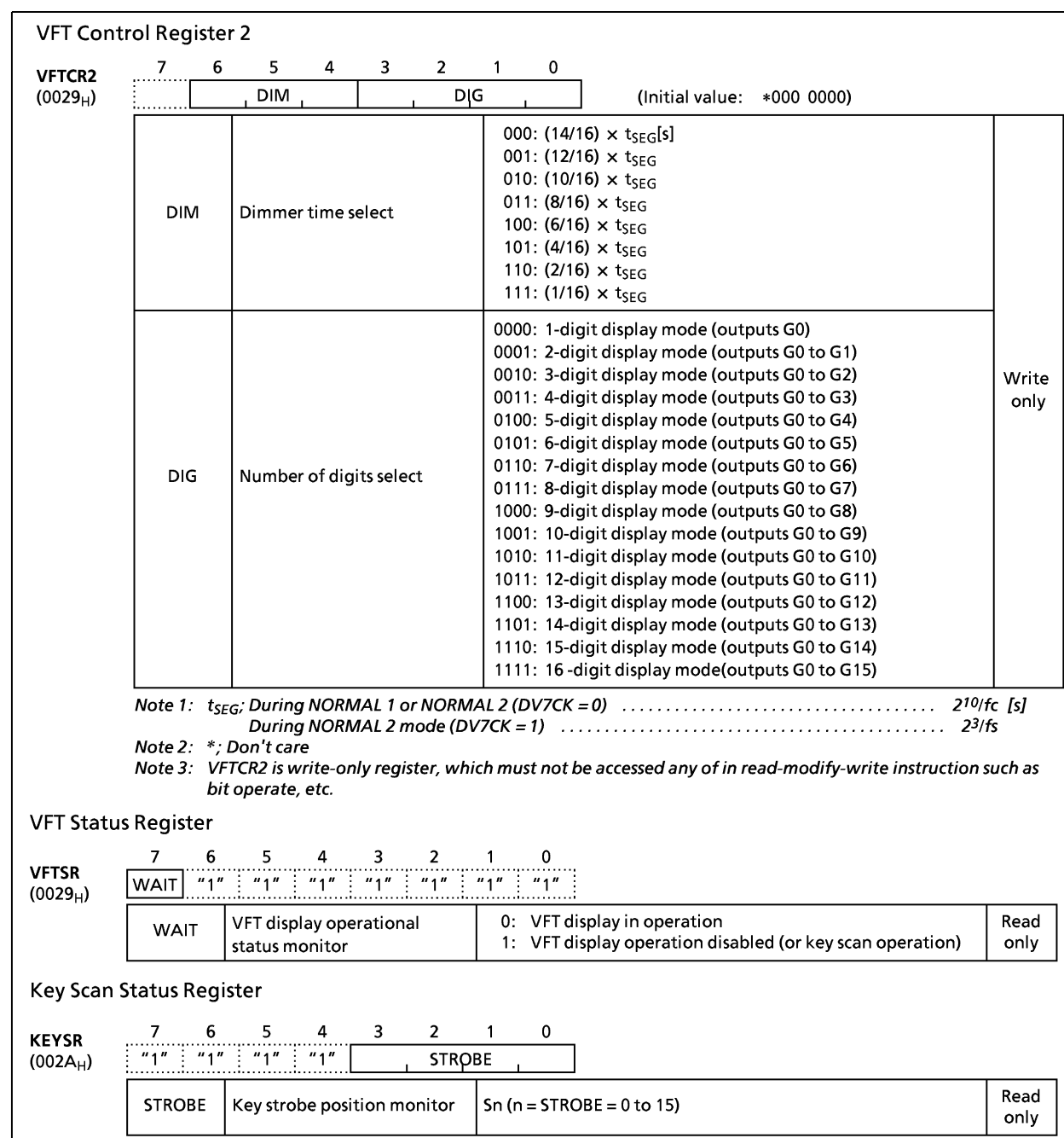
Figure 2-44 (b). VFT Control Registers/Status Registers
