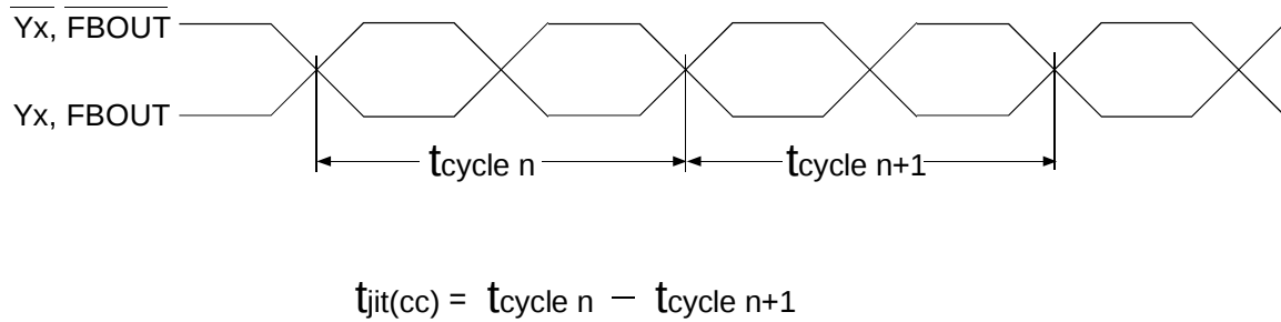
Figure 3. Cycle-to-Cycle jitter
