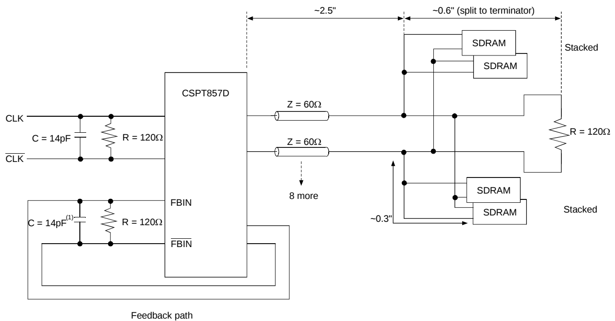
Figure 10. Clock Structure 2
