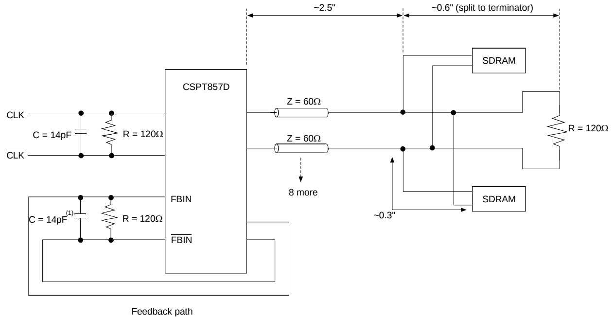
Figure 9. Clock Structure 1
