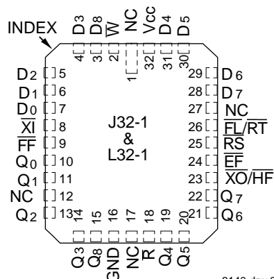
PLCC/LCC TOP VIEW
