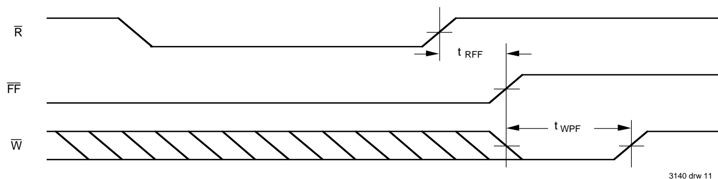
Figure 8. Minimum Timing for an Full Flag Coincident Write Pulse.
