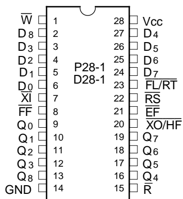
DIP TOP VIEW
