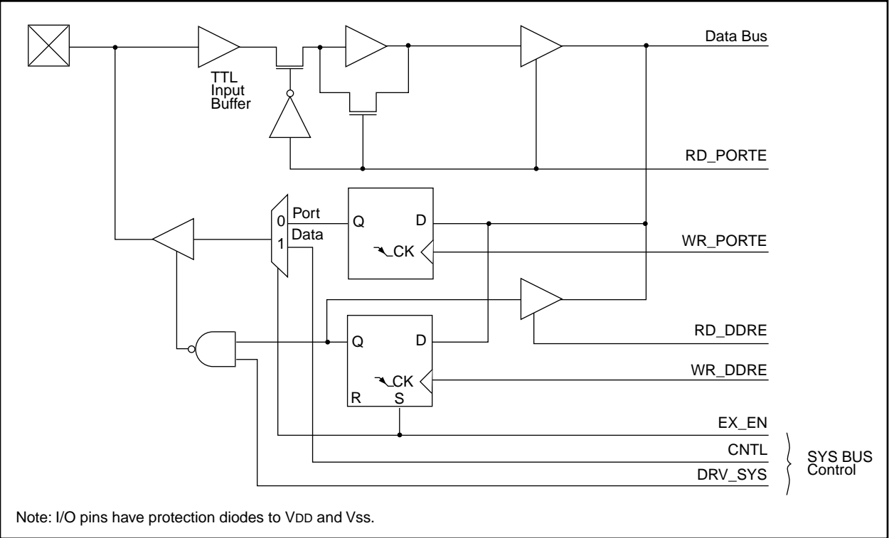
FIGURE 9-8: PORTE BLOCK DIAGRAM (IN I/O PORT MODE)
