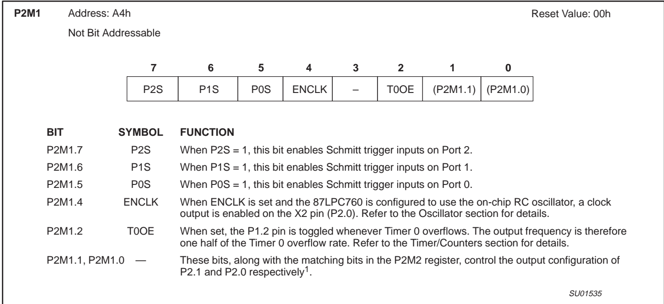
Figure 6. Port 2 Mode Register 1 (P2M1)
