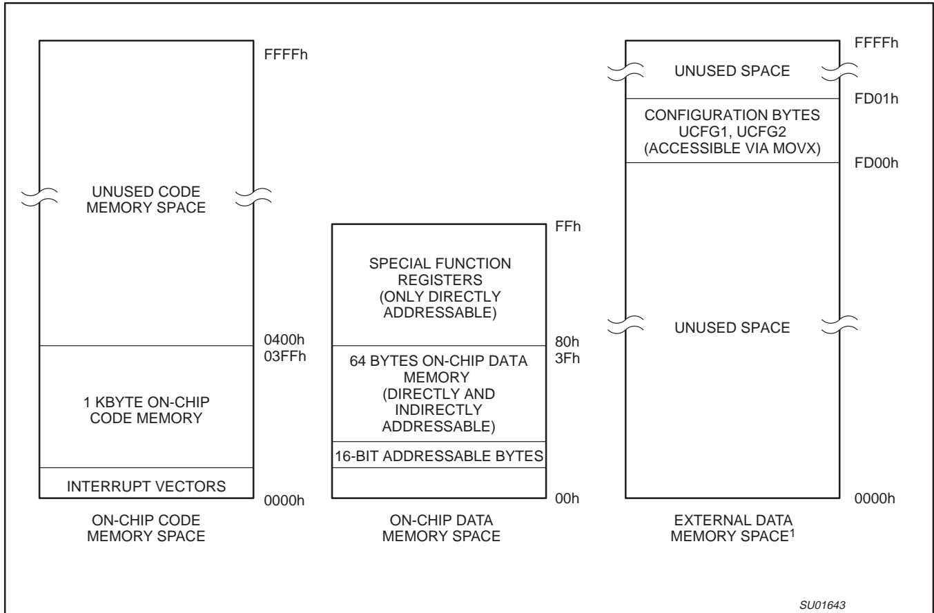
Figure 1. P87LPC759 Program and Data Memory Map
