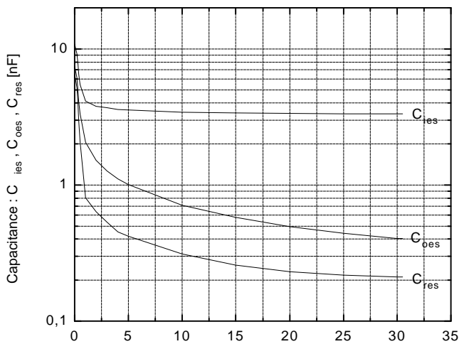
Capacitance vs. Collector-Emitter voltage
