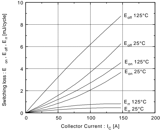
Switching loss vs. Collector current V_{CC}=300V, R_G=24\Omega, V_{GE}=\pm 15V
