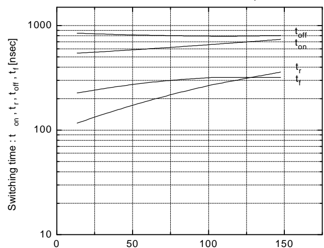
Switching time vs. Collector current V_{CC}=300\text{V}, R_G=24\Omega, V_{GE}=\pm 15\text{V}, T_j=125^\circ\text{C}
