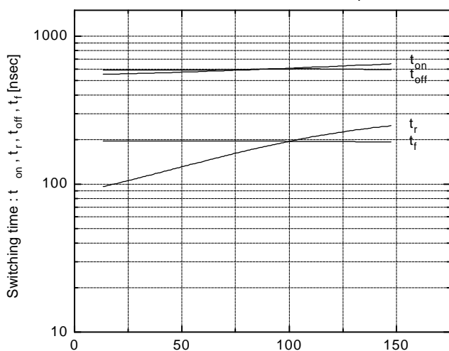
Switching time vs. Collector current V_{CC}=300\text{V}, R_G=24\Omega, V_{GE}=\pm 15\text{V}, T_j=25^\circ\text{C}
