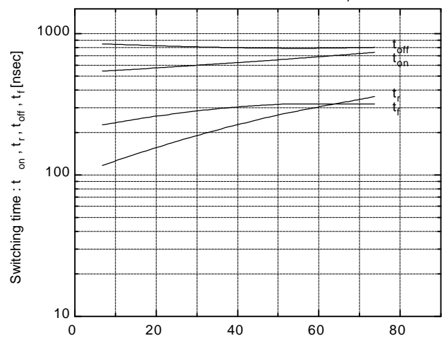
Switching time vs. Collector current V_{CC}=300\text{V}, R_G=51\Omega, V_{GE}=\pm 15\text{V}, T_j=125^\circ\text{C}
