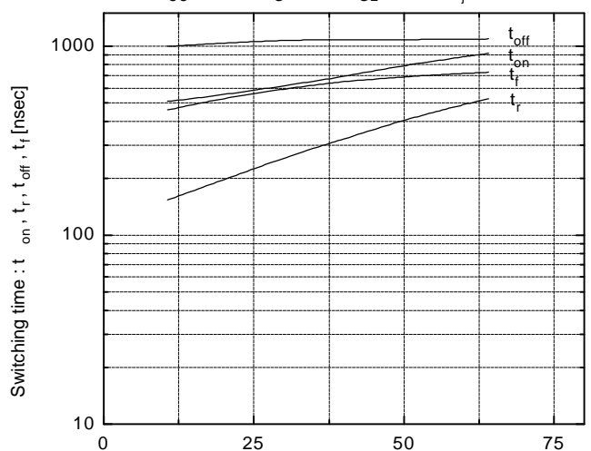
Switching time vs. Collector current V_{CC}=600\text{V}, R_G=24\Omega, V_{GE}=\pm 15\text{V}, T_j=125^\circ\text{C}
