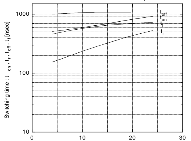
Switching time vs. Collector current
