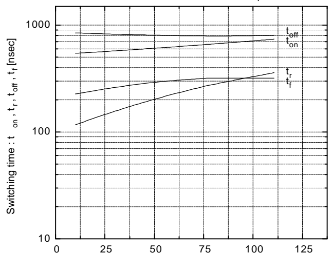
Switching time vs. Collector current V_{CC}=300\text{V}, R_G=33\Omega, V_{GE}=\pm 15\text{V}, T_j=125^\circ\text{C}
