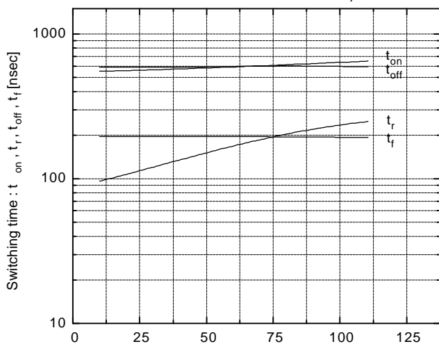
Switching time vs. Collector current V_{CC}=300\text{V}, R_G=33\Omega, V_{GE}=\pm 15\text{V}, T_j=25^\circ\text{C}
