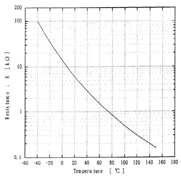
[ Thermistor ] Temperature characteristic (typ.)
