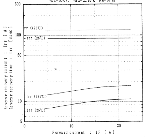
[ Inverter ] Reverse recovery characteristics (typ.) V_{ce} = 80 \text{OV} , V_{GE} = \pm 15 \text{V} , R_g = 82 \Omega
