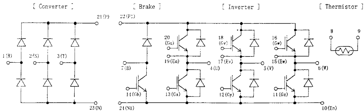
2. Equivalent circuit
