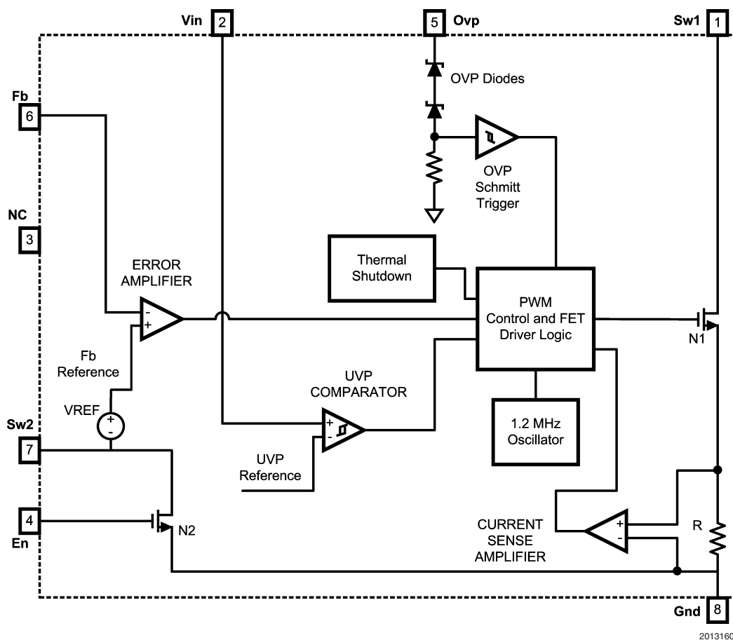
FIGURE 2. Block Diagram
