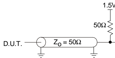
Figure 21 Output Test Load
