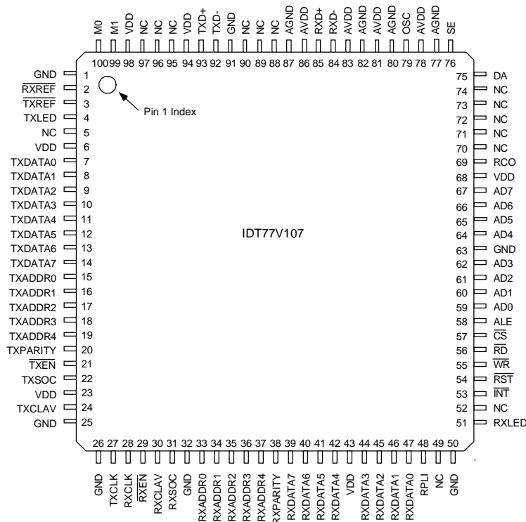
Figure 1 Pin Assignments
