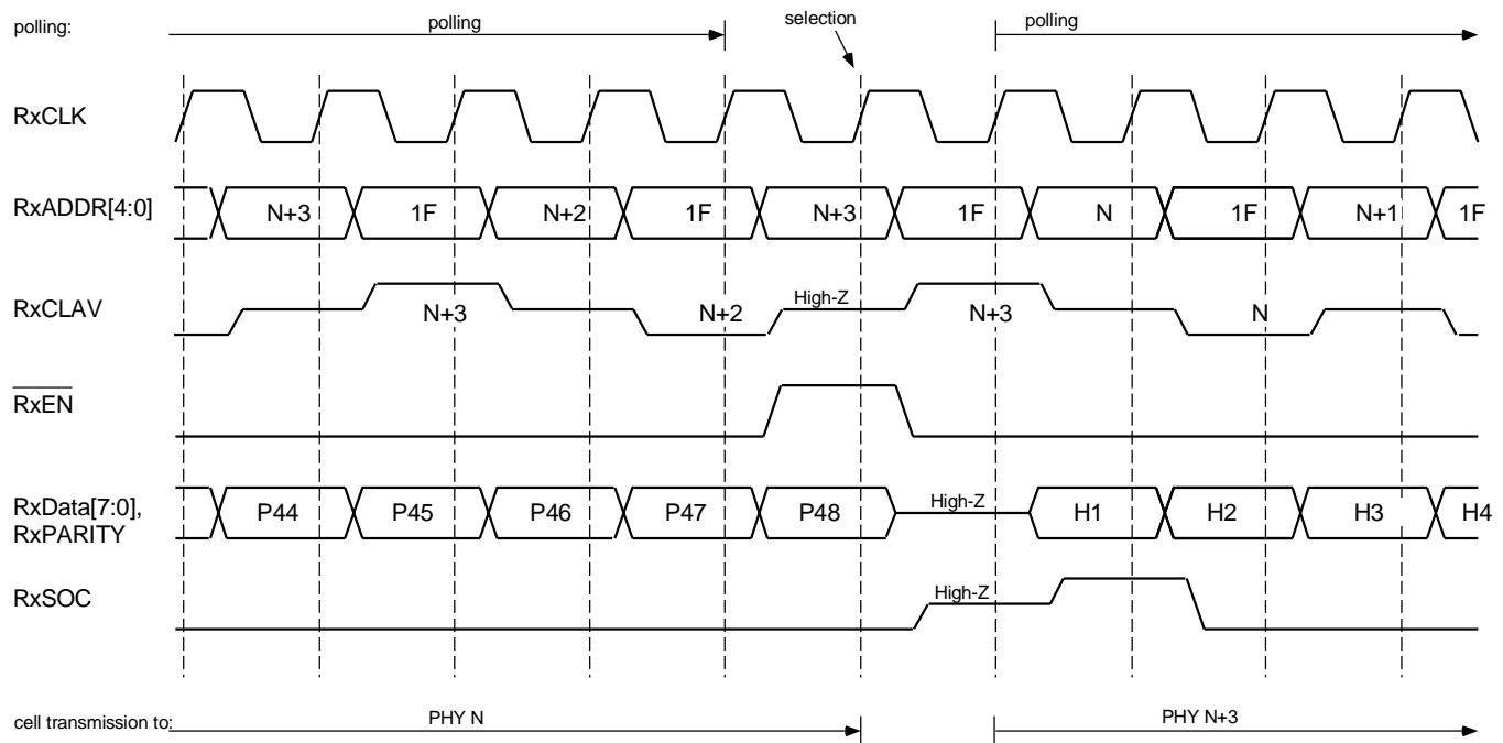
Figure 8 Utopia Receive Handshake - Back to Back Cells
