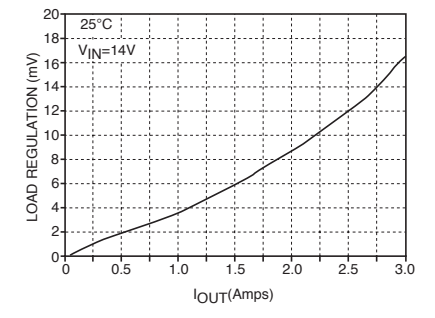
Load Regulation vs. I_{OUT}
