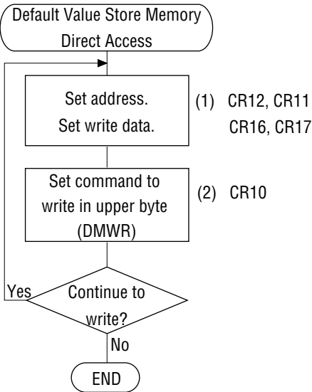
Figure 8-1 Flow Chart of Default Value Store Memory Direct Access
