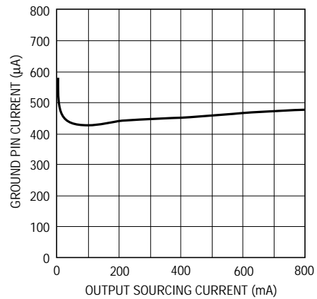
Ground Pin Current vs Output Source Current
