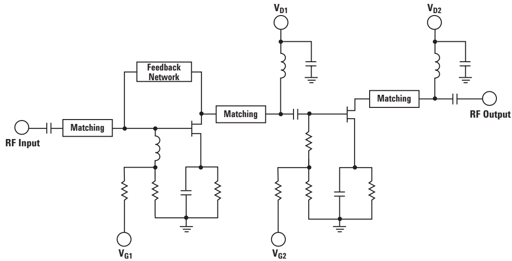
Figure 18. AMMC-5618 Schematic
