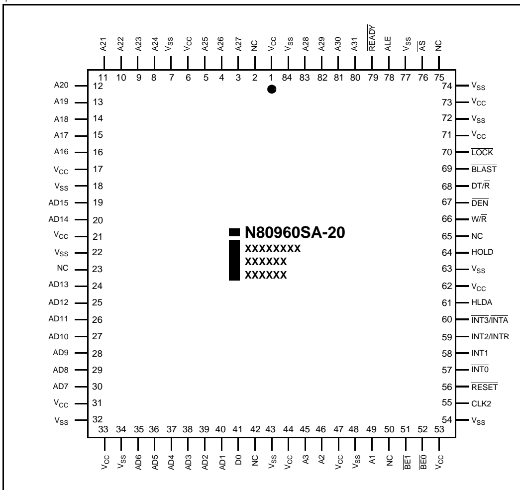
Figure 16. 84-Lead Plastic Leaded Chip Carrier (PLCC) Package
