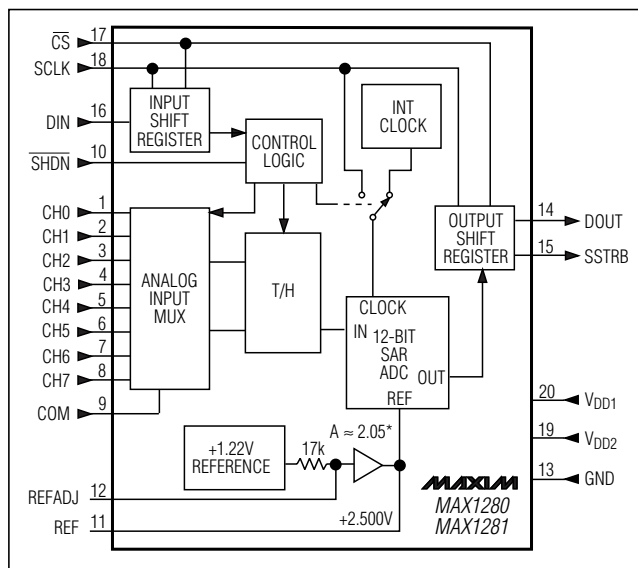
Figure 3. Functional Diagram
