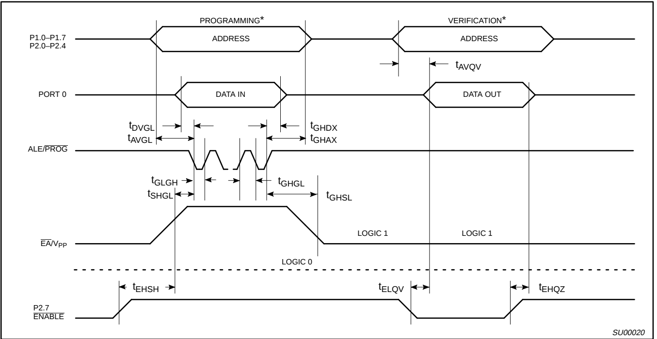
Figure 28. EPROM Programming and Verification
