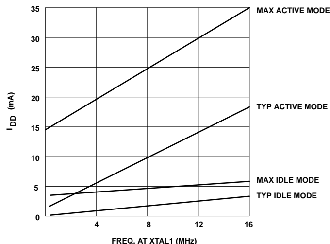
I_{DD} vs. FREQUENCY
