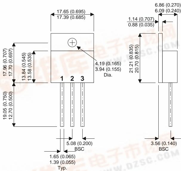
TO-258 Package Outline. Dimensions in mm (inches)
