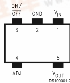
5-Lead Small Outline Package (M5)
