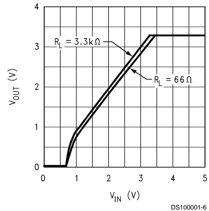
Dropout Characteristics
