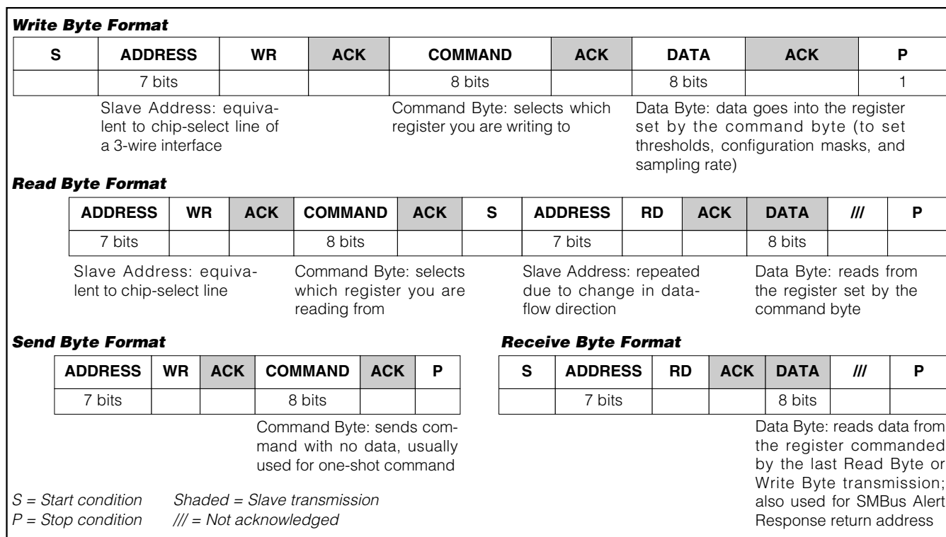
Figure 3. SMBus Protocols
