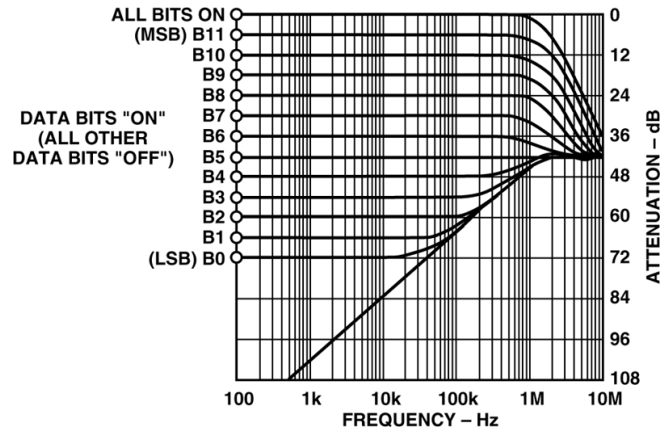
FIGURE 2. MULTIPLYING MODE FREQUENCY RESPONSE VS. DIGITAL CODE
