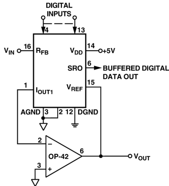
FIGURE 20. ANALOG/DIGITAL DIVIDER
