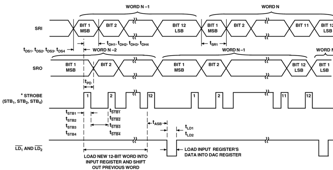
FIGURE 15. TIMING DIAGRAM
