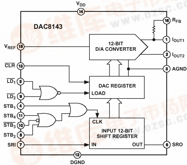
Logic Diagram
