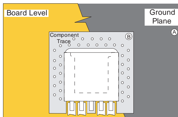
Figure 3 – Recommended Layout
