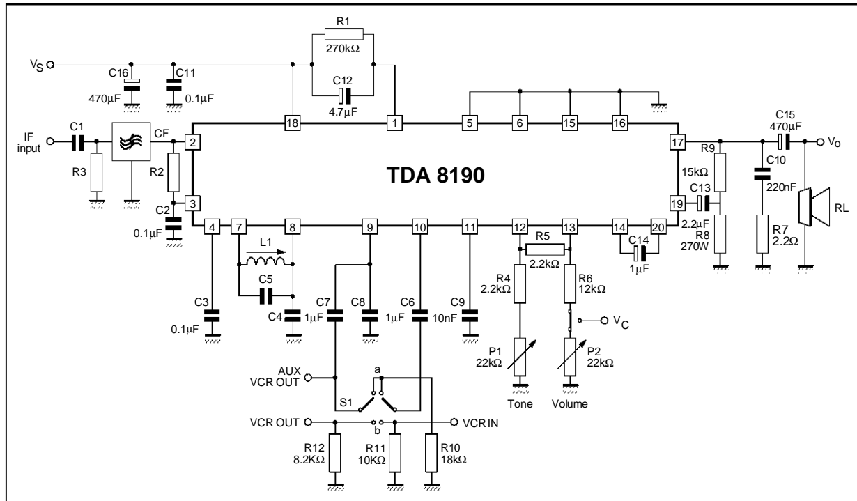
Figure 16 : Application Circuit
