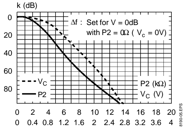
Figure 4 : Amplitude Modulation Rejection versus Input Signal
