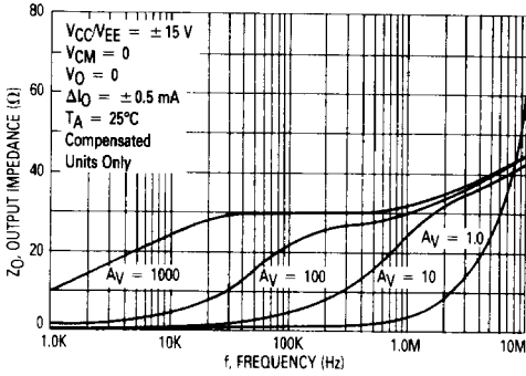
FIGURE 9 — OUTPUT IMPEDANCE versus FREQUENCY
