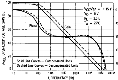
FIGURE 14 — OPEN-LOOP VOLTAGE GAIN AND PHASE versus FREQUENCY
