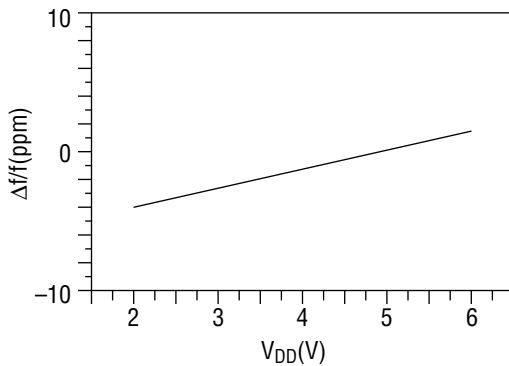
Supply voltage dependency of oscillation frequency
