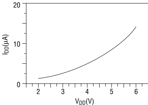
Supply voltage dependency of I_{DD}
