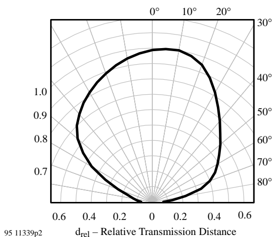
Figure 13. Vertical Directivity \varphi_y
