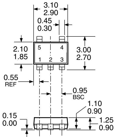
Dwg. MA-011-5 mm
