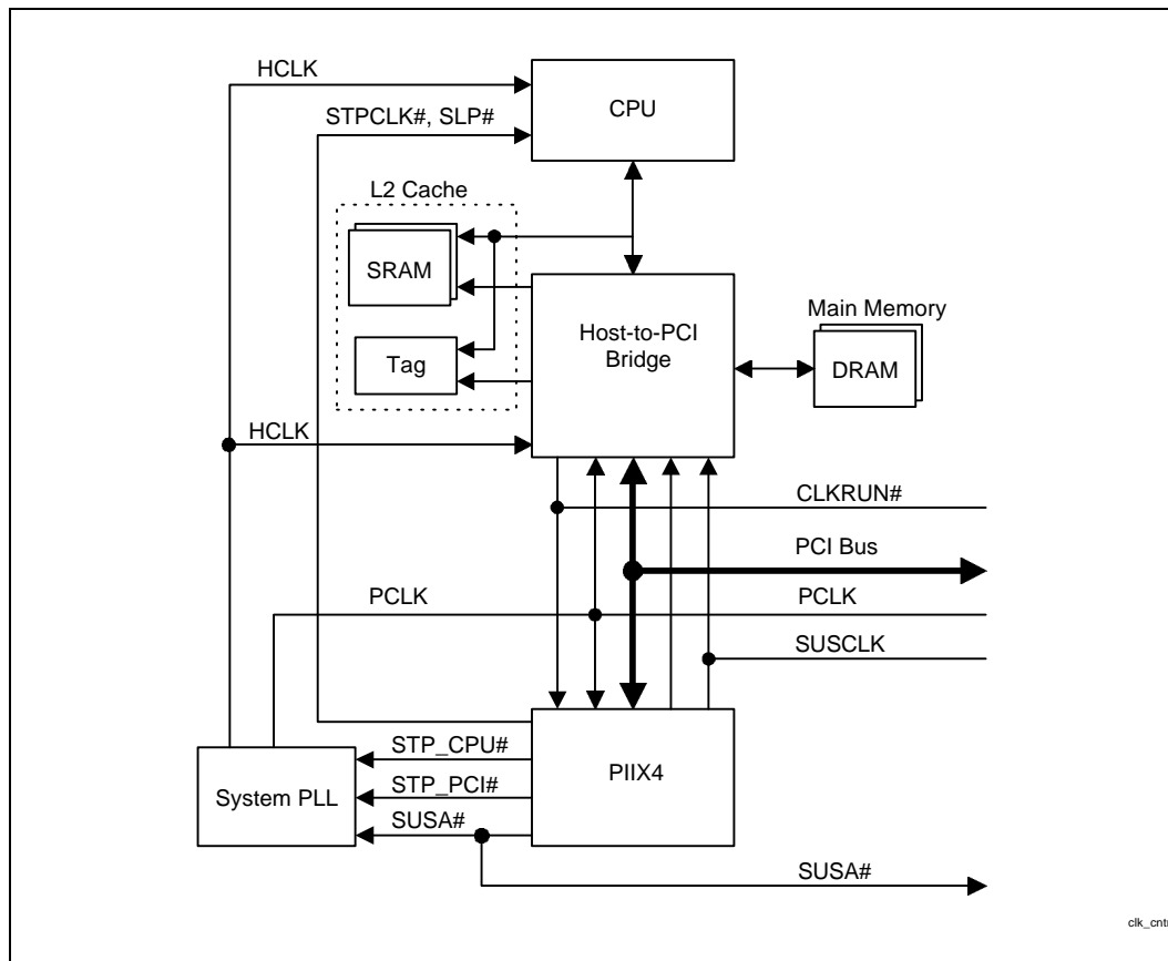
Figure 10. Clock Control
