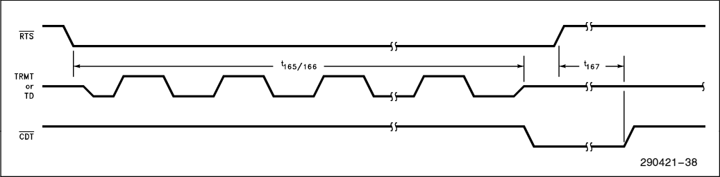
Figure 39. Jabber Timings
