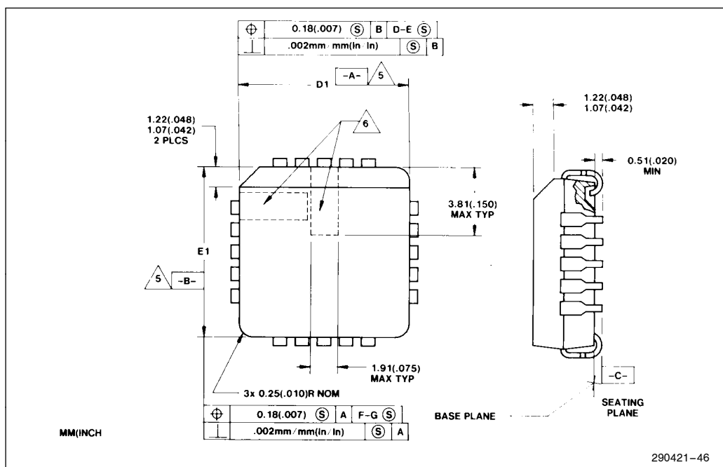
Figure 46. Molded Details
