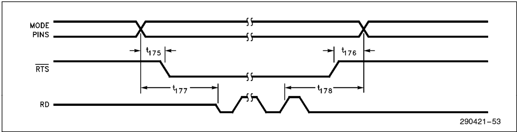
Figure 41. Mode Timings
