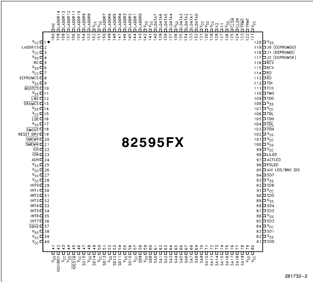
Figure 2. 82595FX Pinout
