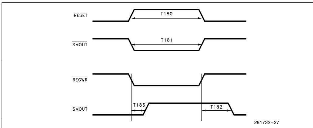
Figure 11-14. \overline{\text{SMOUT}} Timing
