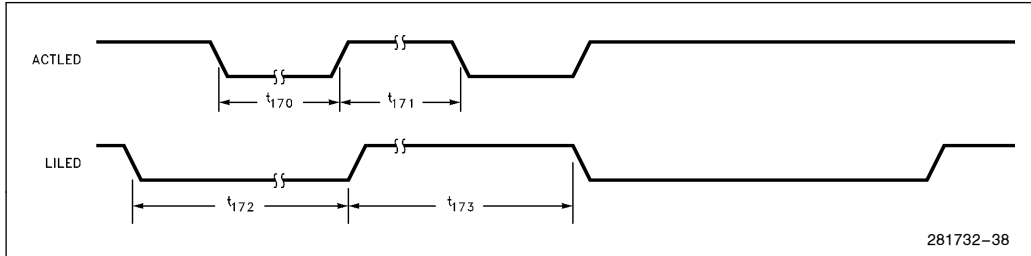
Figure 11-24. LED Timings
