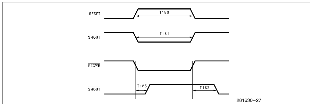
Figure 11-17. \overline{\text{SMOUT}} Timing
