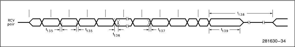
Figure 11-23. AUI Receive Timings
