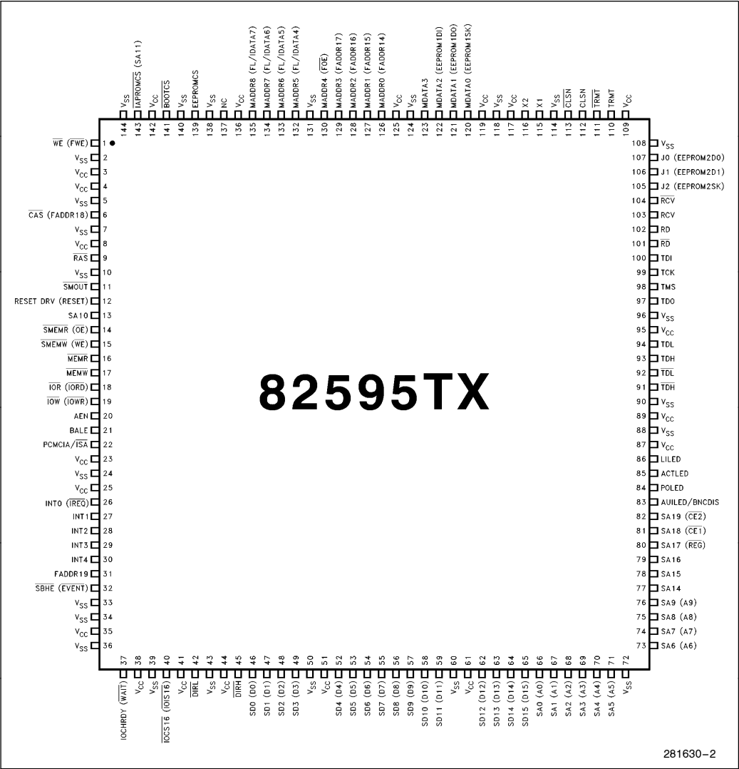
Figure 2. 82595TX Pinout
