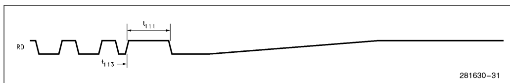
Figure 11-20. TPE Receive Timings (End of Frame)
