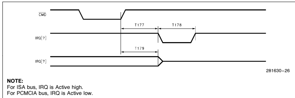
Figure 11-16. Interrupt Timing
