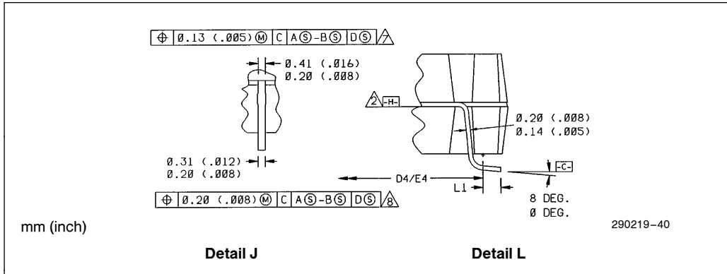
Figure 64. Typical Lead
