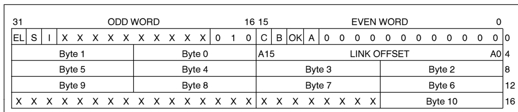
Figure 23. CONFIGURE—82586 Mode
