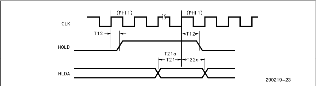
Figure 50. HOLD/HLDA Timings
