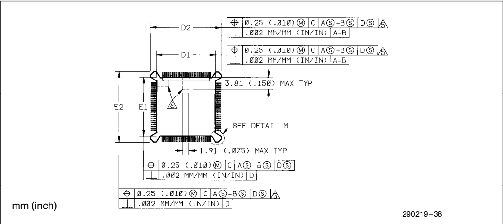
Figure 62. Molded Details
