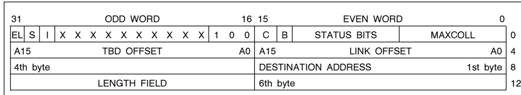
Figure 28. TRANSMIT—82586 Mode
