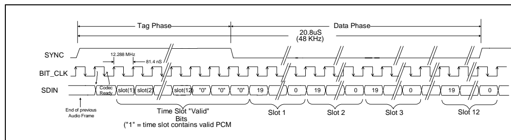
Figure 5-19. AC-link Protocol
