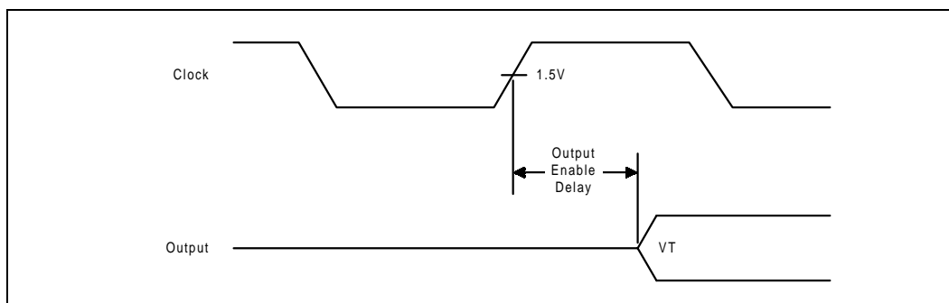
Figure 14-6. Output Enable Delay
