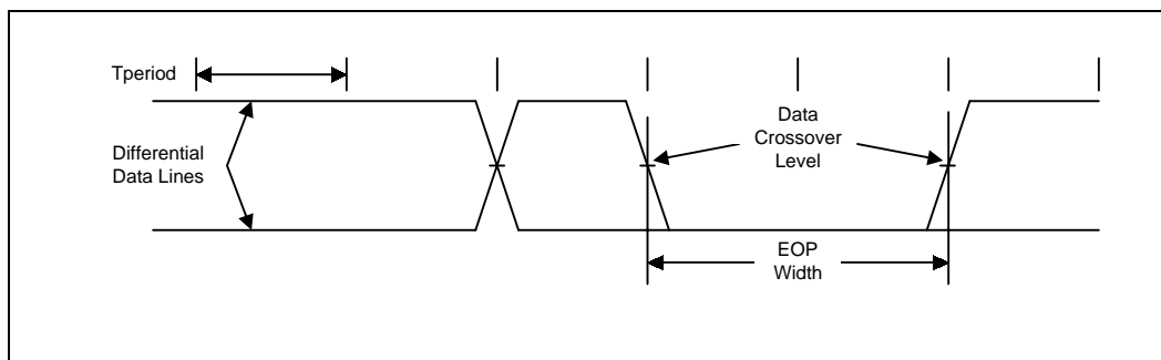
Figure 14-16. SMBus Transaction
