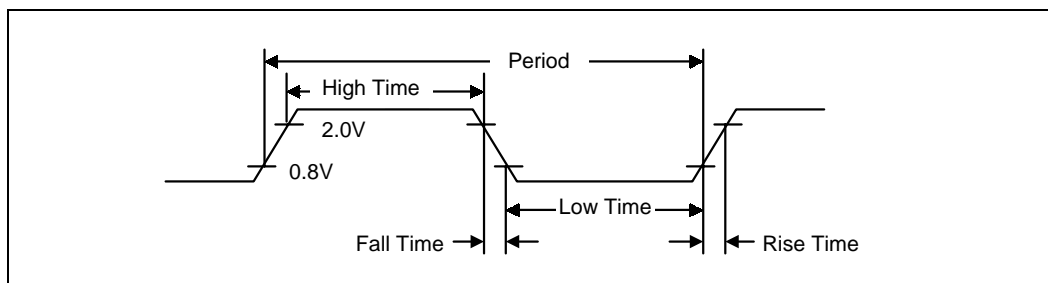
Figure 14-1. Clock Timing
