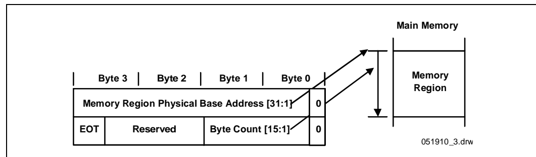
Figure 5-14. Physical Region Descriptor Table Entry
