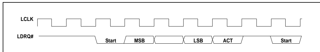
Figure 5-11. DMA Request Assertion Through LDRQ#
