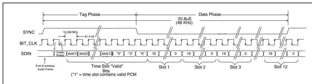
Figure 5-22. AC-Link Protocol
