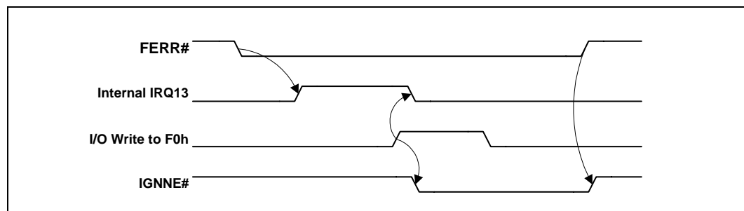
Figure 5-12. Coprocessor Error Timing Diagram
