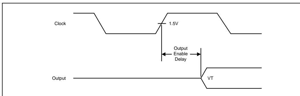
Figure 17-6. Output Enable Delay
