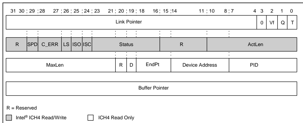
Figure 5-15. Transfer Descriptor
