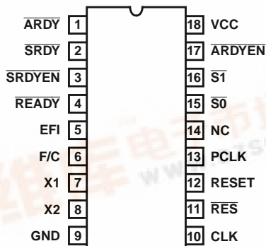
82C284 (CERDIP) TOP VIEW
