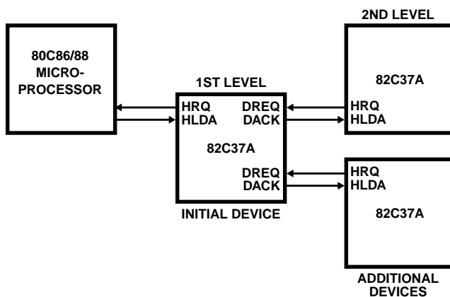
FIGURE 3. CASCADED 82C37As
