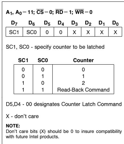
Figure 9. Counter Latching Command Format
