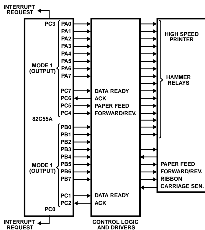
FIGURE 18. PRINTER INTERFACE
