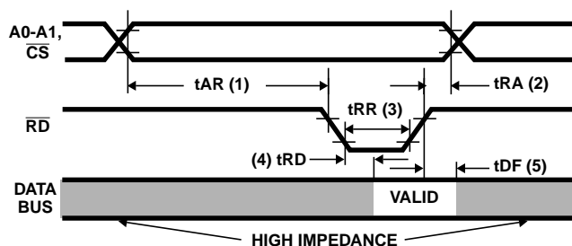
FIGURE 31. READ TIMING
