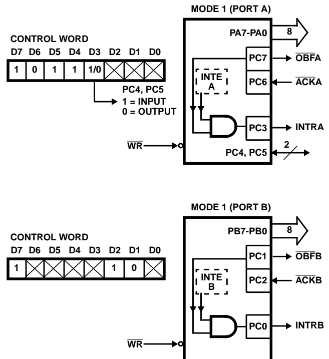
FIGURE 8. MODE 1 OUTPUT
