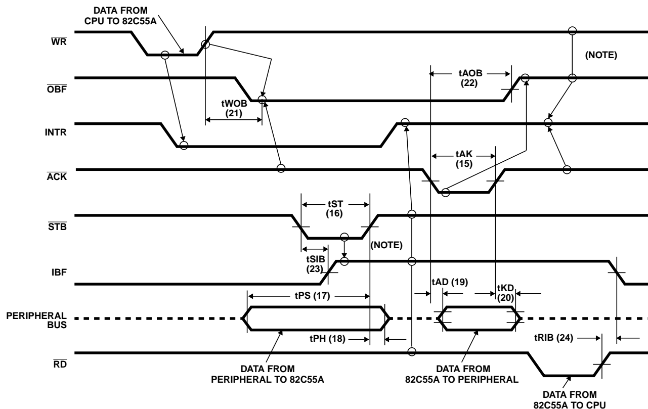
FIGURE 29. MODE 2 (BI-DIRECTIONAL)
