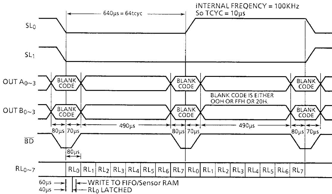
Figure 12.4 Scan Timing
