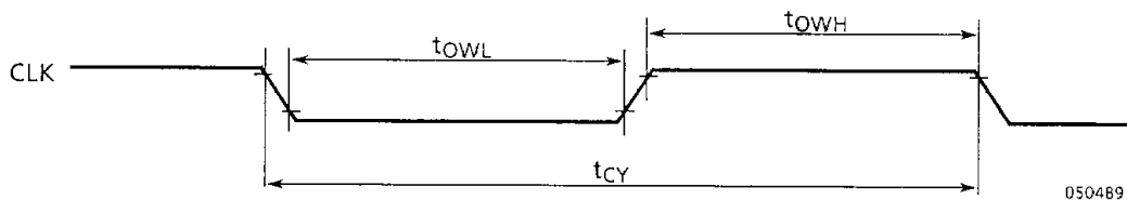
Figure 12.3 CLOCK TIMING
