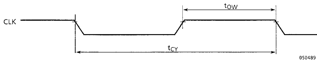
Figure 12.3 Clock Timing
