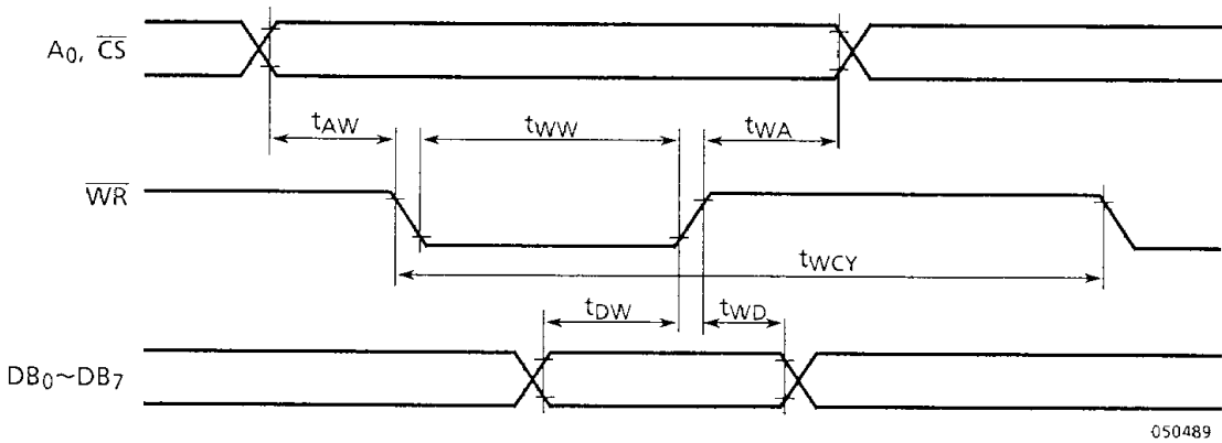
Figure 12.2 WRITE TIMING
