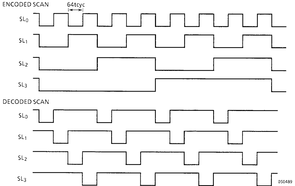
Figure 12.4 Scan Timing
