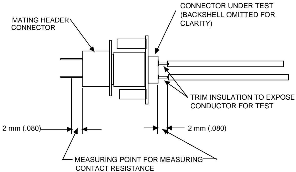
FIGURE 1 CONTACT RESISTANCE MEASUREMENT
