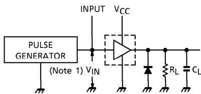
7. t_{ON}, t_{OFF}
