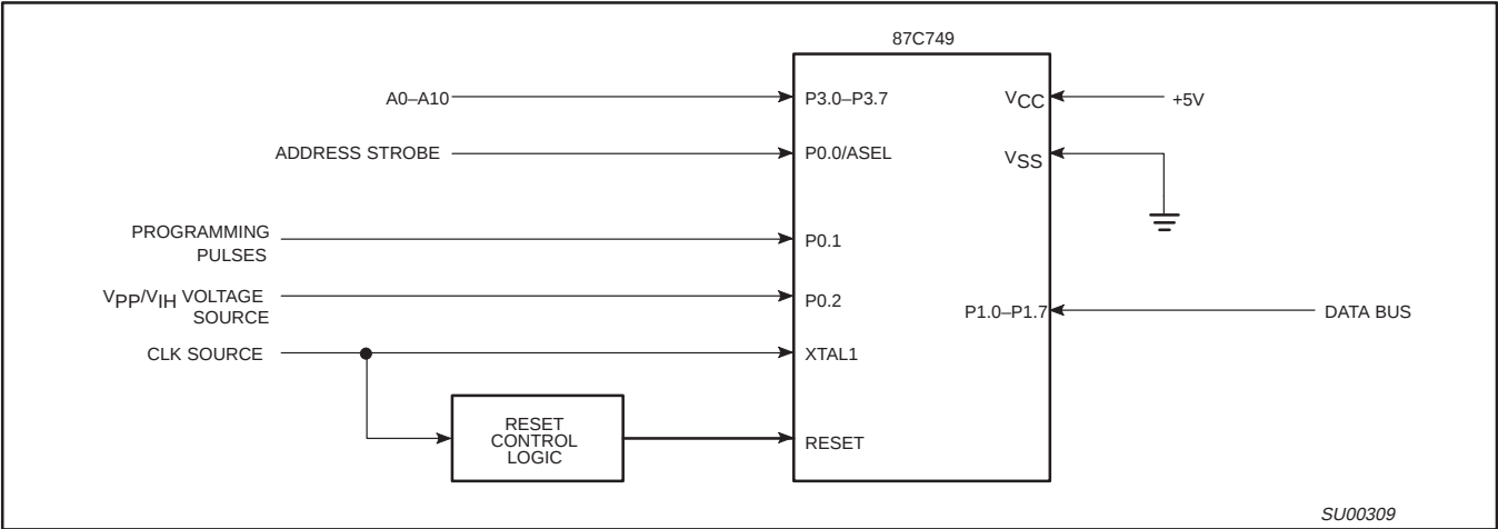
Figure 7. Programming Configuration
